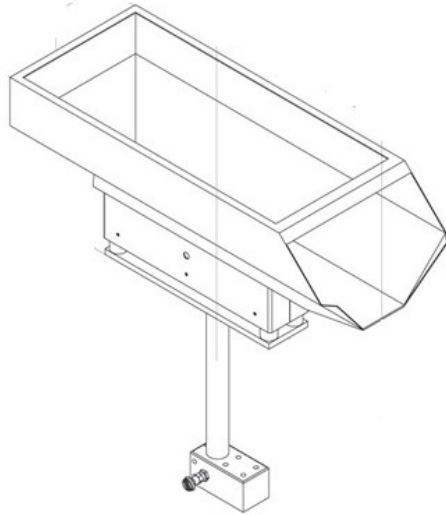
Vibratory Hopper
